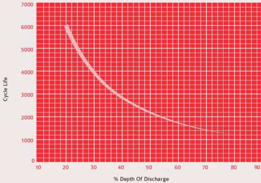
CYCLE LIFE VERSUS DOD FOR 12V GEL
