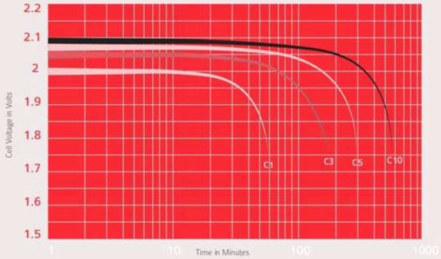
PERFORMANCE CURVES AT DIFFERENT RATES OF DISCHARGE
